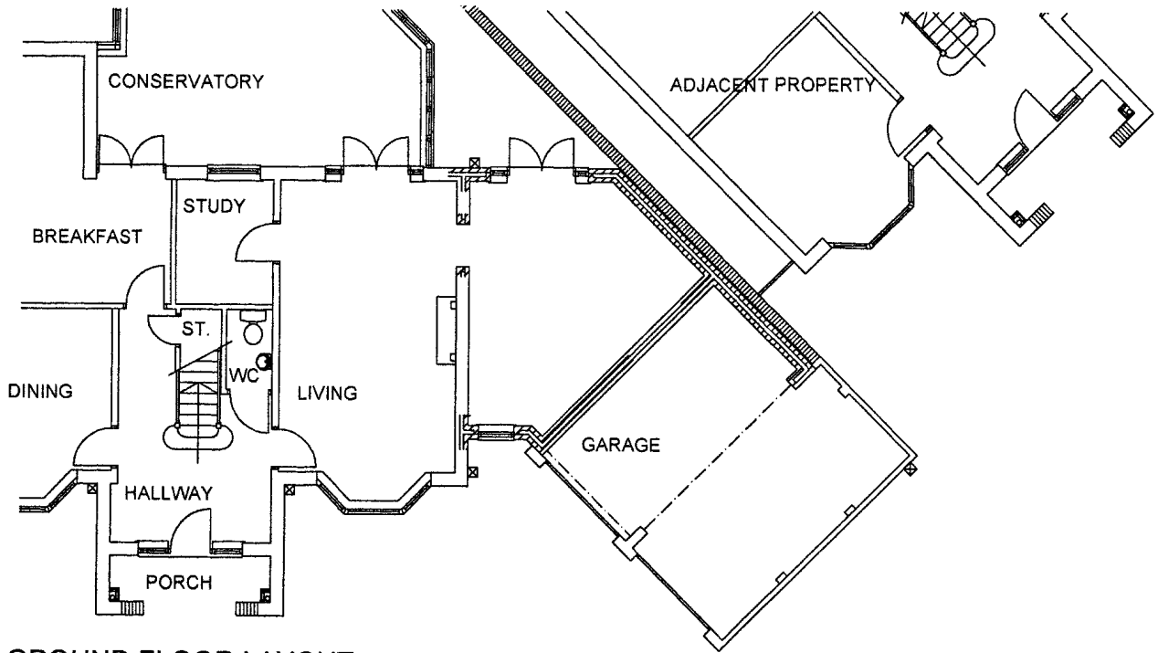
GROUND FLOOR LAYOUT
